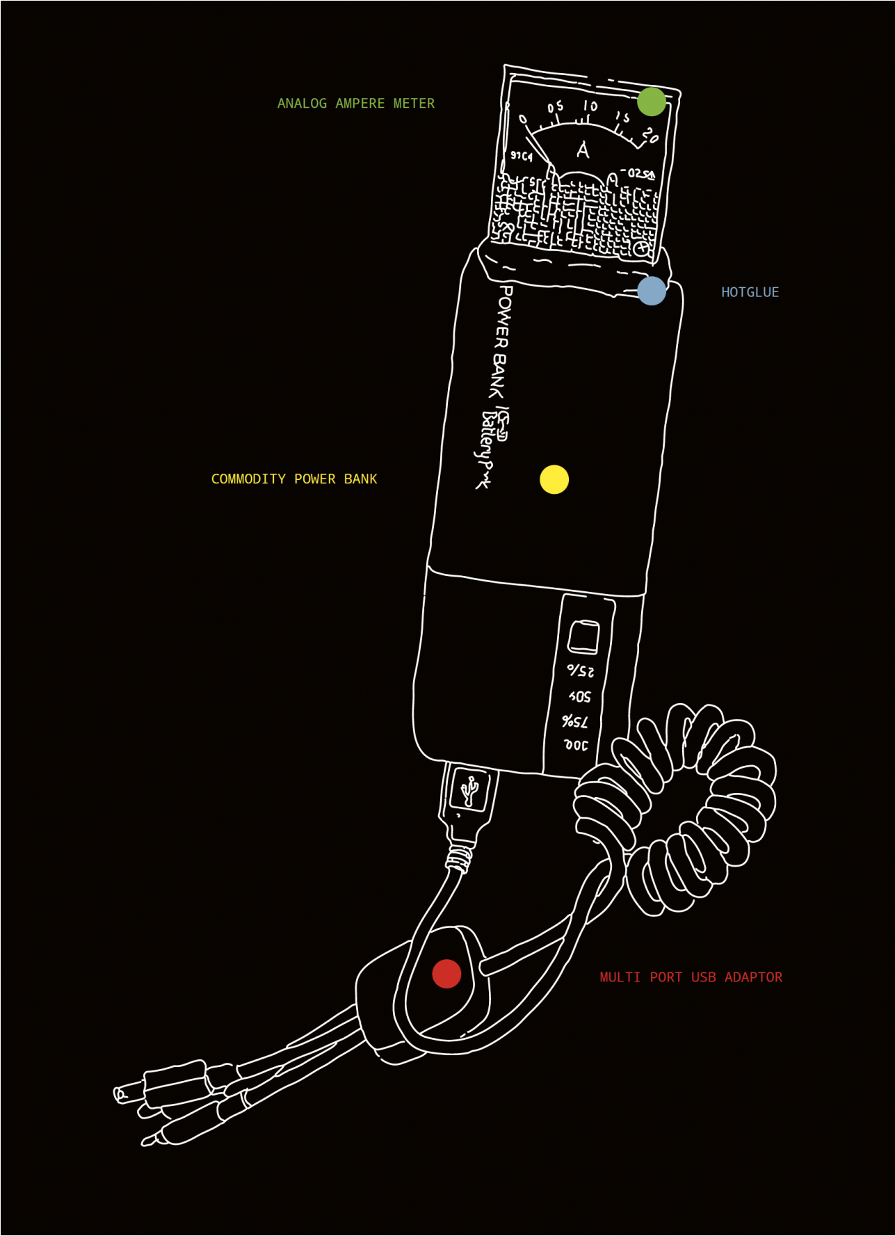
Figure 1.6 Diagram of a portable charging test power supply.
